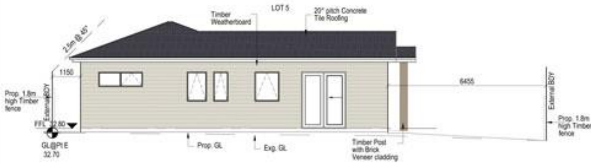
SOUTHERN ELEVATION A Scale: 1 : 100
